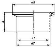
WELDING CLAMP FIG.1712
